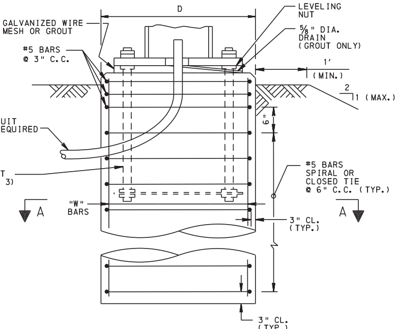
TYPE A FOUNDATION CASE 1
