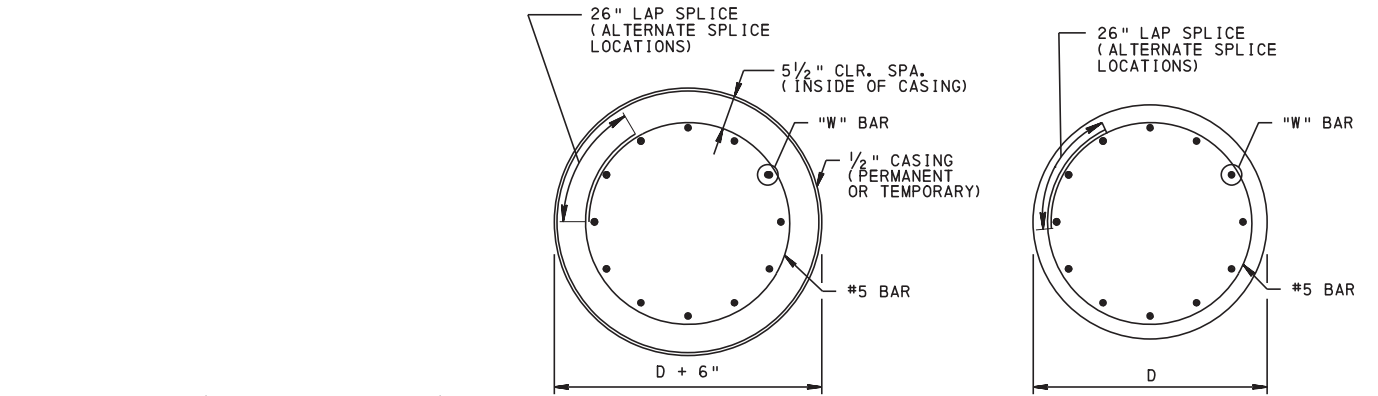
CLOSED TIE DETAILS CASES 3 AND 4
