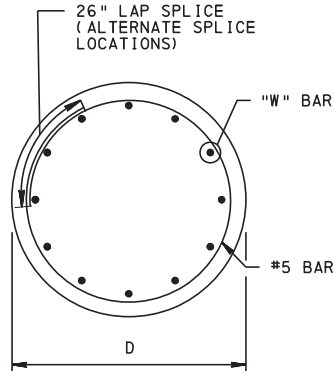
CLOSED TIE DETAIL CASES 1 AND 2
