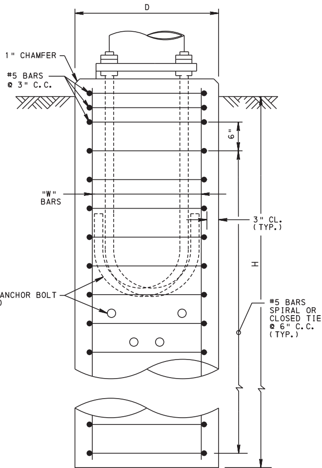
SECTION
