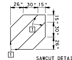
DETECTOR SAWCUT DETAIL
