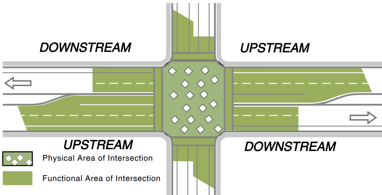
Figure 3: Physical and Functional Area of Intersection (FHWA-SA-10-002)
