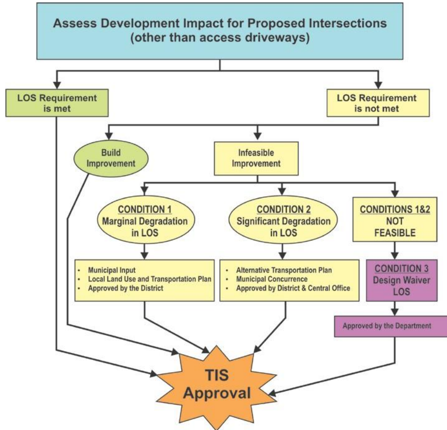
Figure 9: Mitigation Procedure
