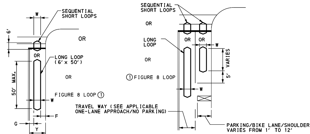
ONE-LANE APPROACH / NO PARKING
