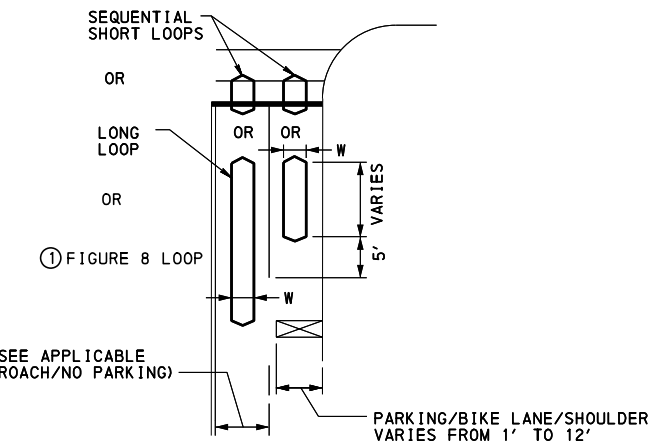
ONE-LANE APPROACH WITH PARKING, BIKE LANE OR SHOULDER (SEE APPLICABLE ONE-LANE APPROACH/NO PARKING)
