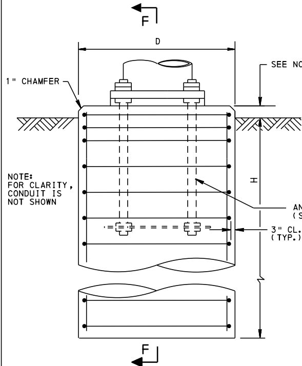
SECTION
