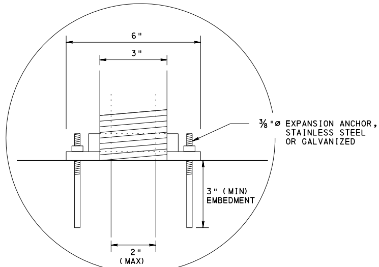
CONNECTION DETAIL
