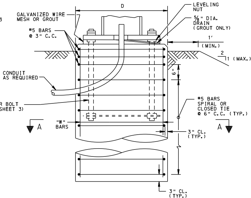
SECTION F-F
