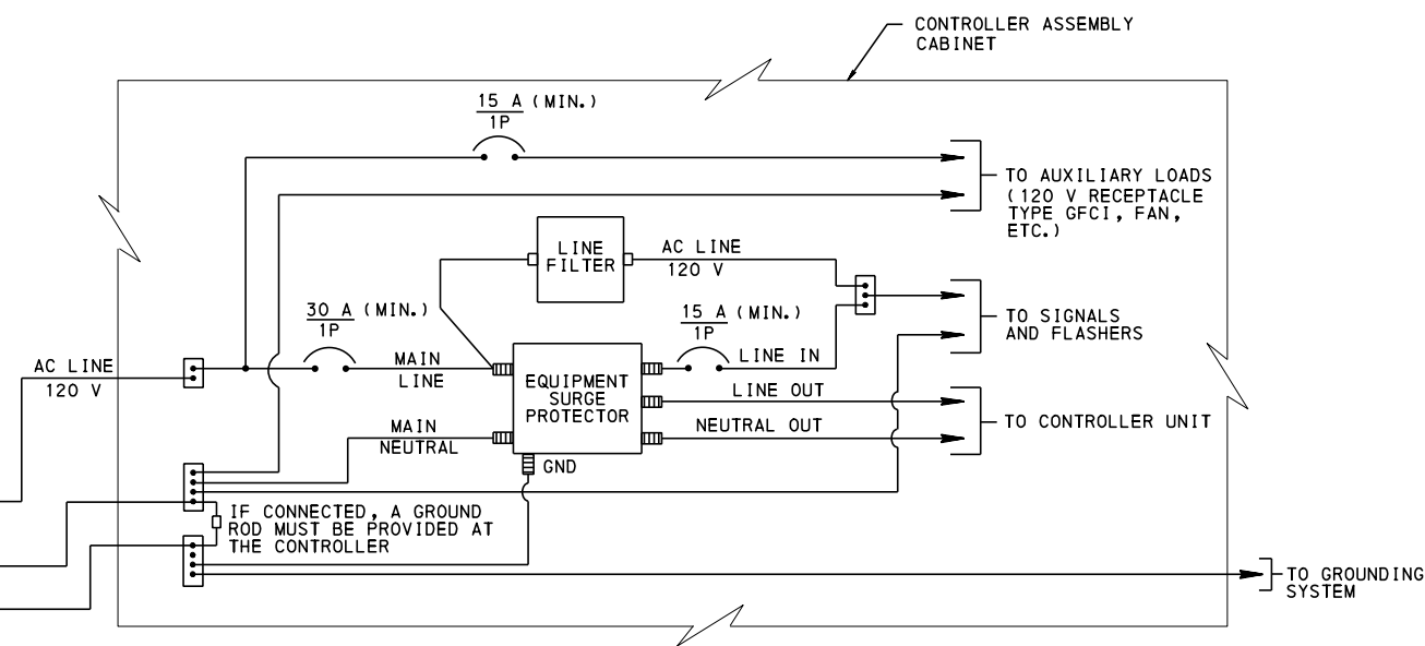
TYPICAL WIRING DIAGRAM
