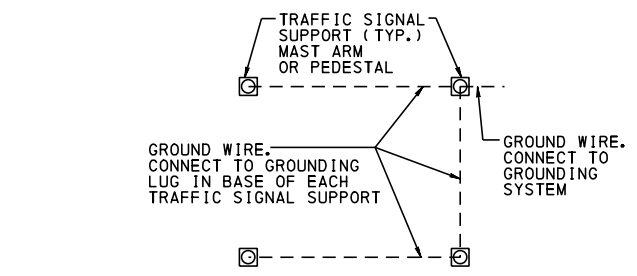
MAST ARM OR PEDESTAL SUPPORT
