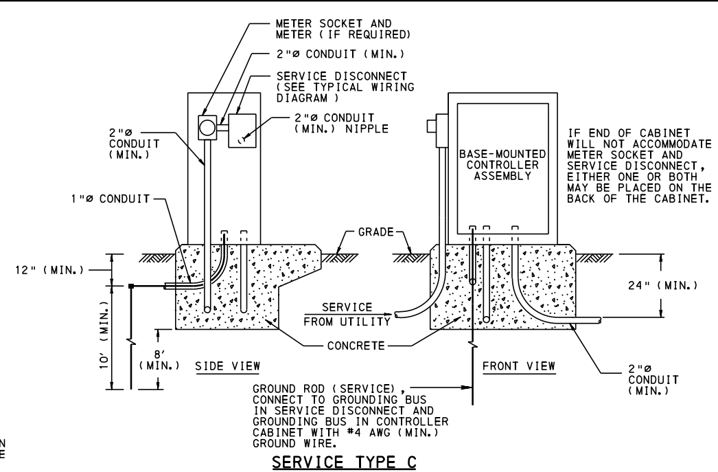
SERVICE TYPE C
