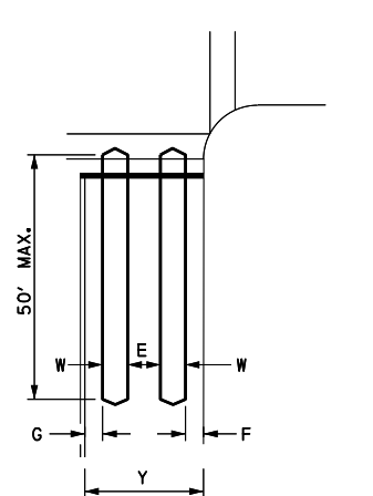
ONE / TWO-LANE APPROACH / NO PARKING
