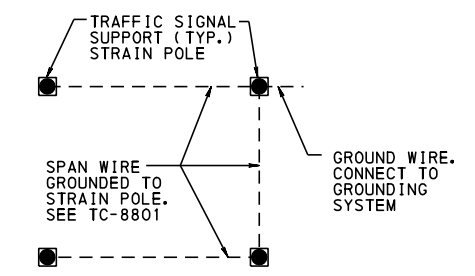
STRAIN POLE SUPPORT
