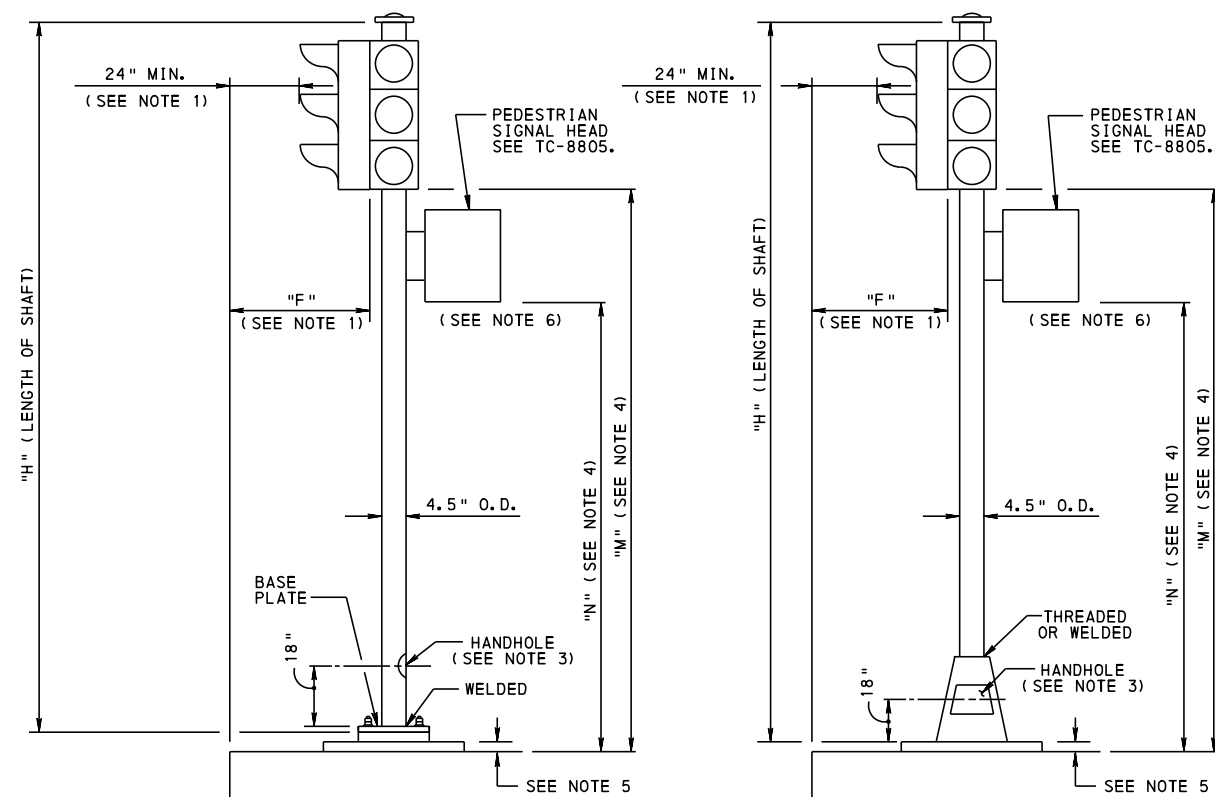
PLATE BASE
