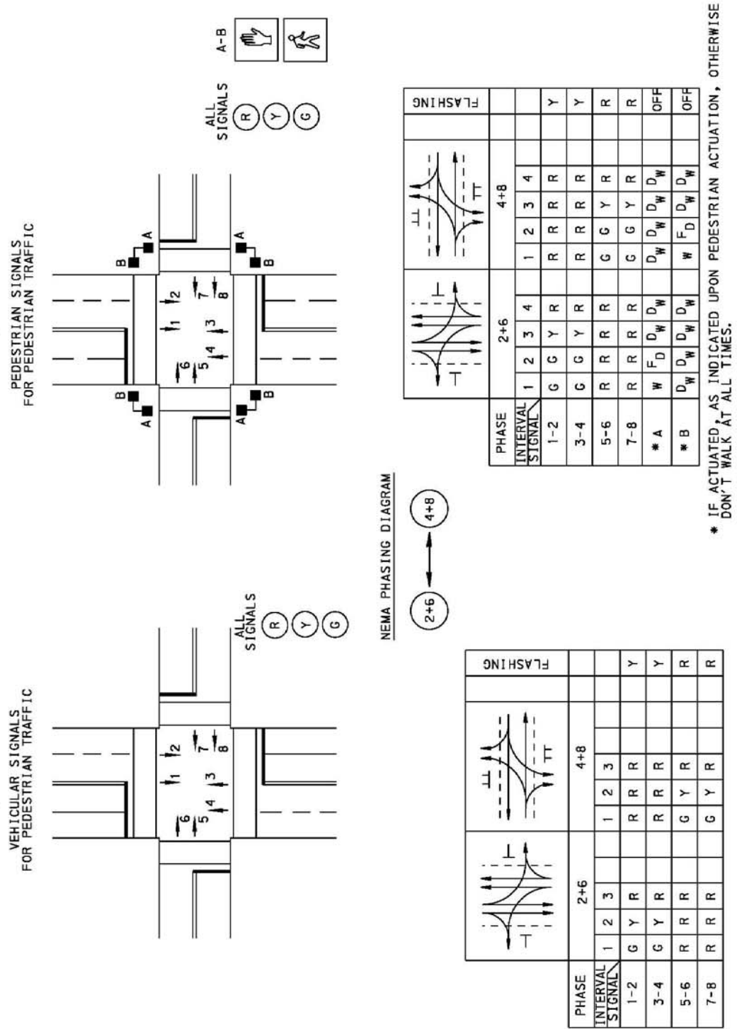
FIGURE A-6 SAMPLE TWO-PHASE OPERATION
