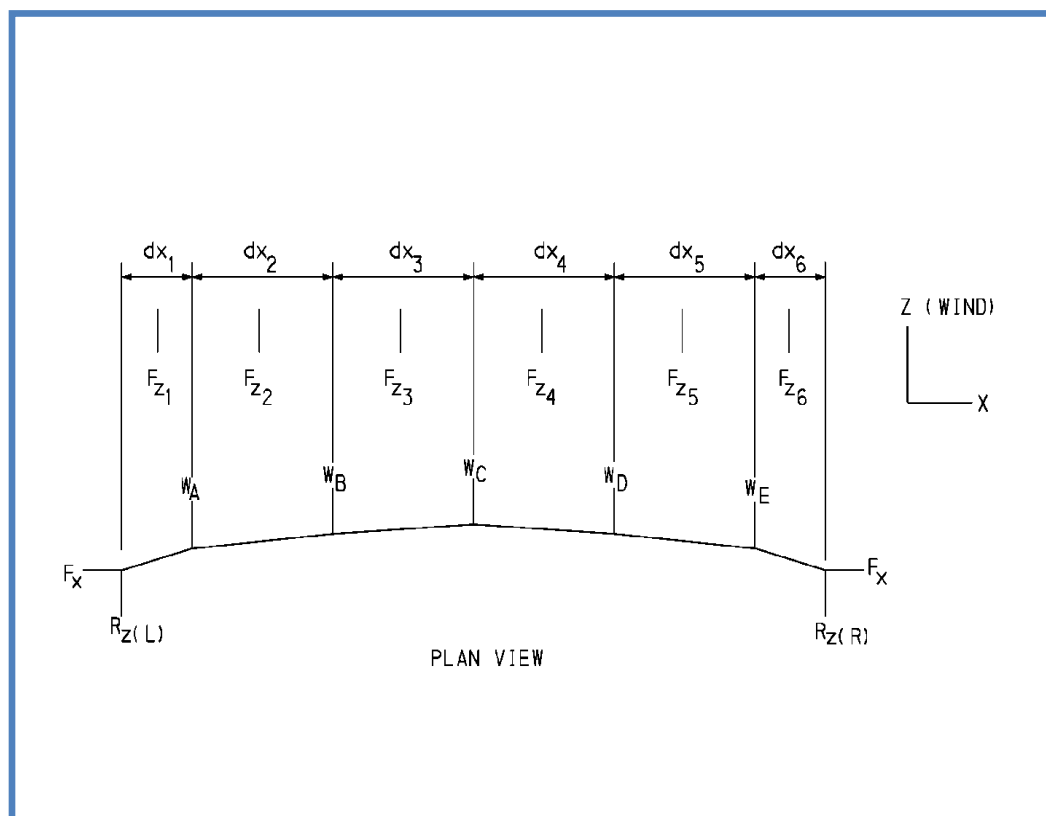
Exhibit 20-1 Force Diagram
