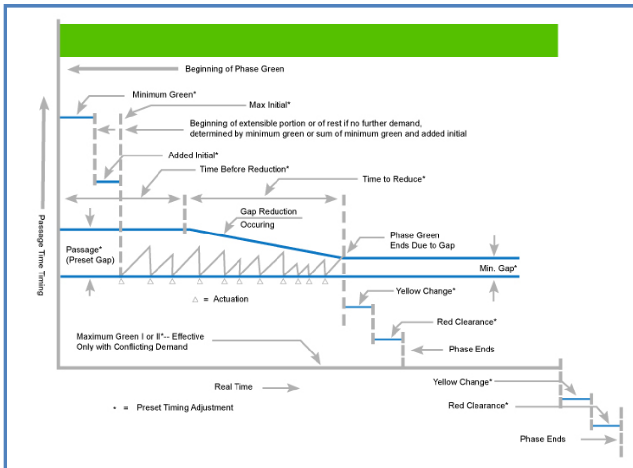
Exhibit 3-9 Volume-Density Operation
