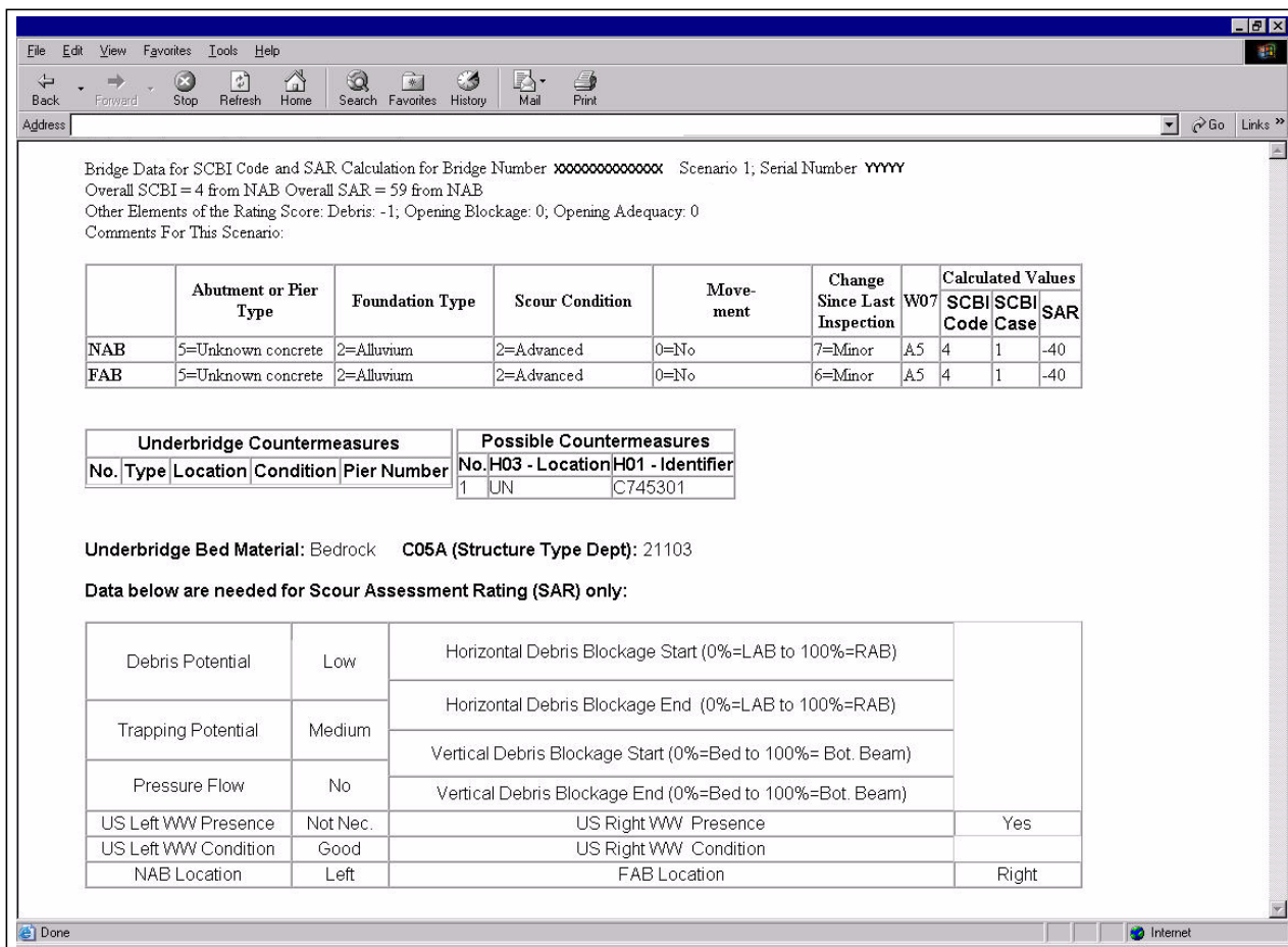
Figure 11. Reformatted printer-friendly page for Scour Critical Bridge Indicator Code and Scour Assessment Rating calculator.
